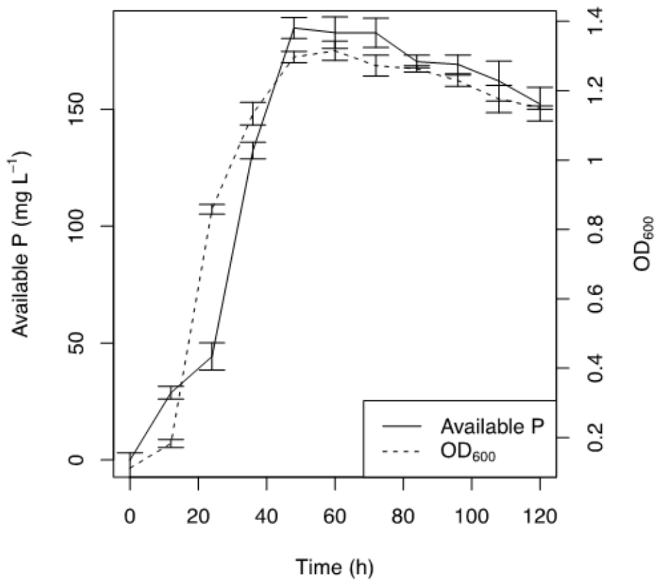
Supplementary figure. Growth profile of Acinetobacter sp. RC04 and culture phosphate solubility. Error bars show standard errors ( n = 5 ). OD_{600} was correlated with P solubilization (Spearman's rank correlation \rho = 0.95 , P < 10^{-16} ).
