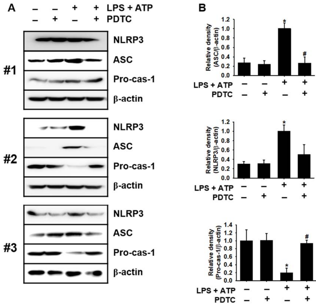
Supplementary Figure S10: Triplicate data (A) and densitometric analysis (B) of Figure 8D.
