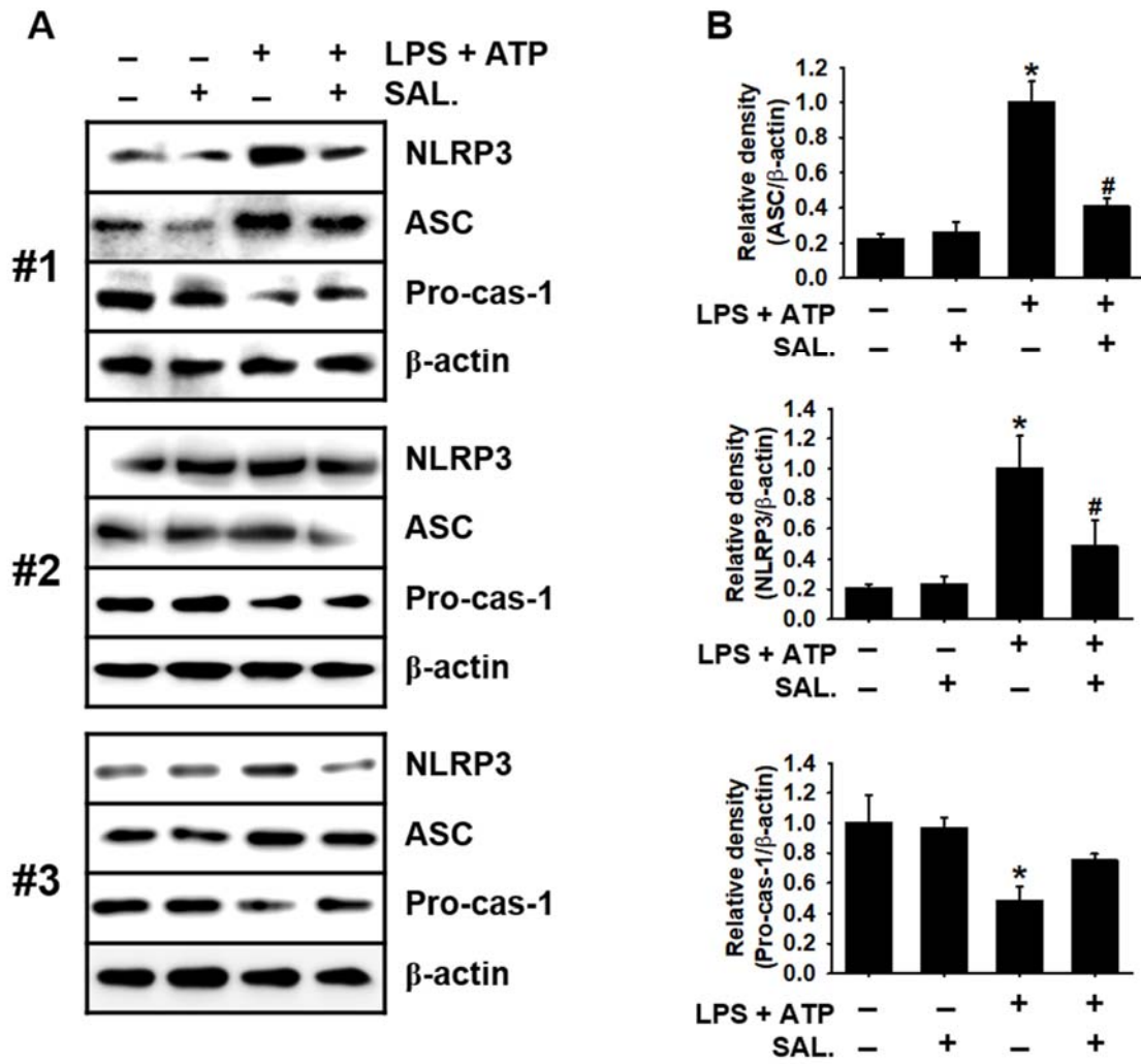
Supplementary Figure S7: Triplicate data (A) and densitometric analysis (B) of Figure 3E.
