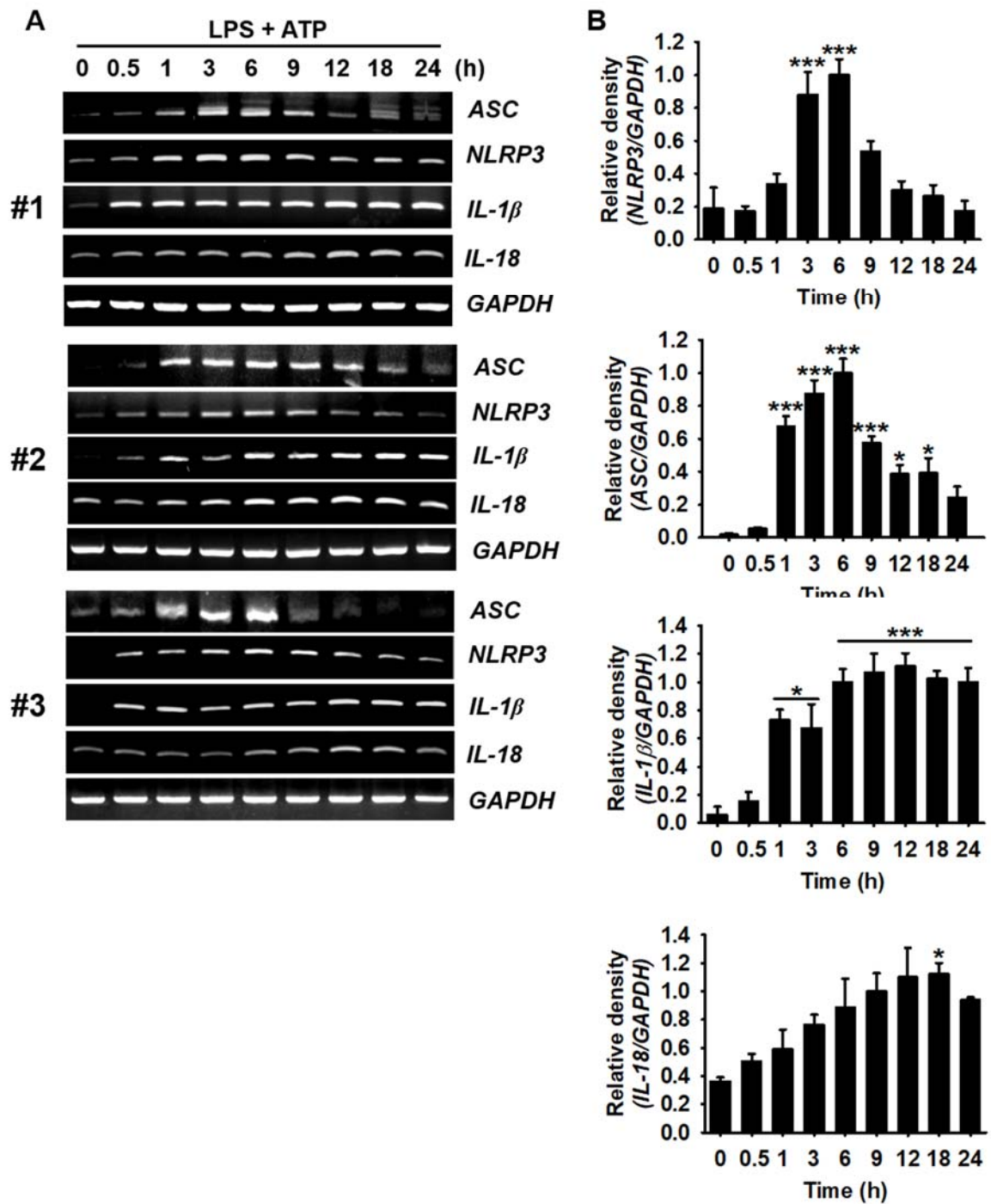
Supplementary Figure S1: Triplicate data (A) and densitometric analysis (B) of Figure 2A.
