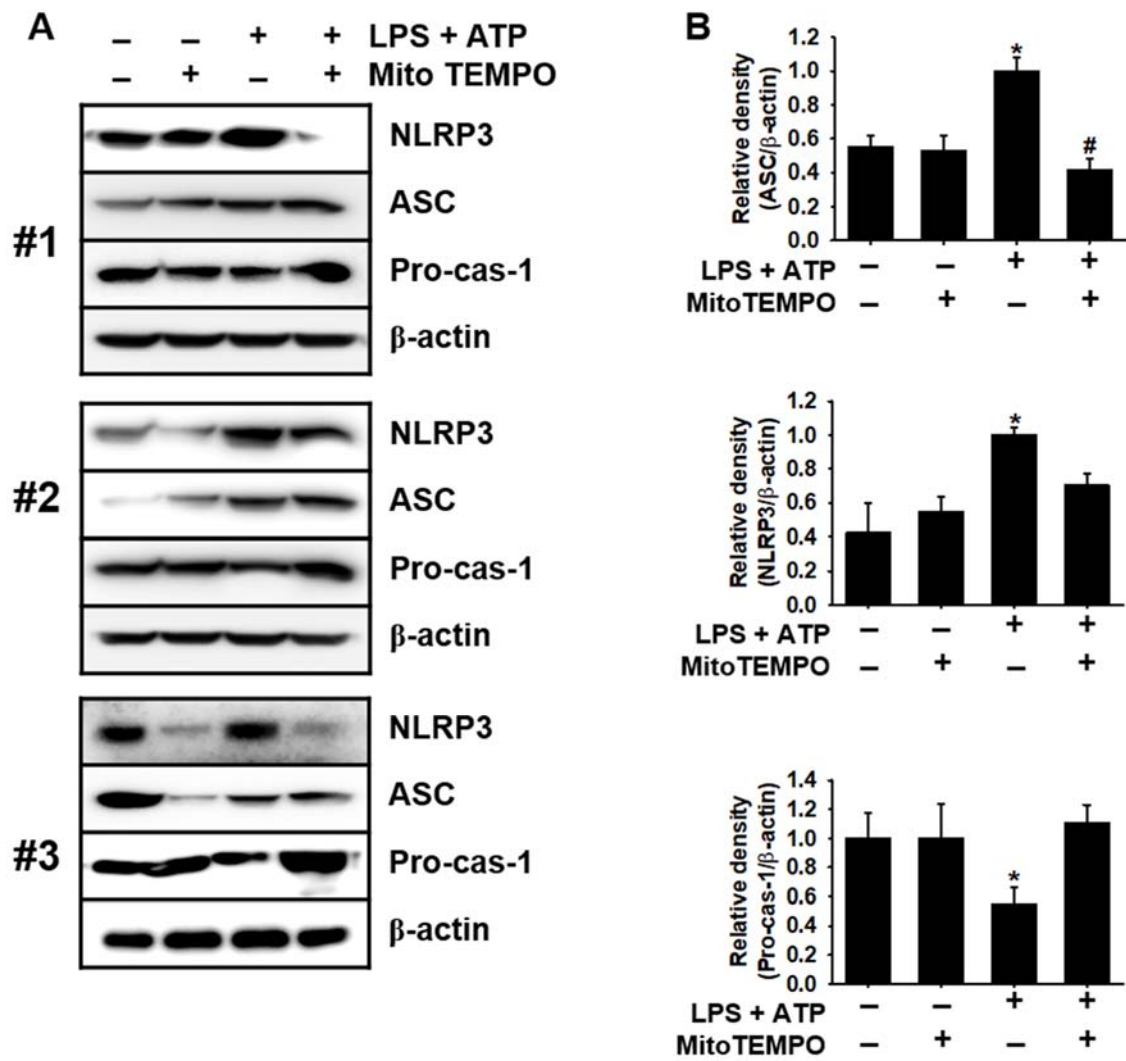
Supplementary Figure S8: Triplicate data (A) and densitometric analysis (B) of Figure 4C.
