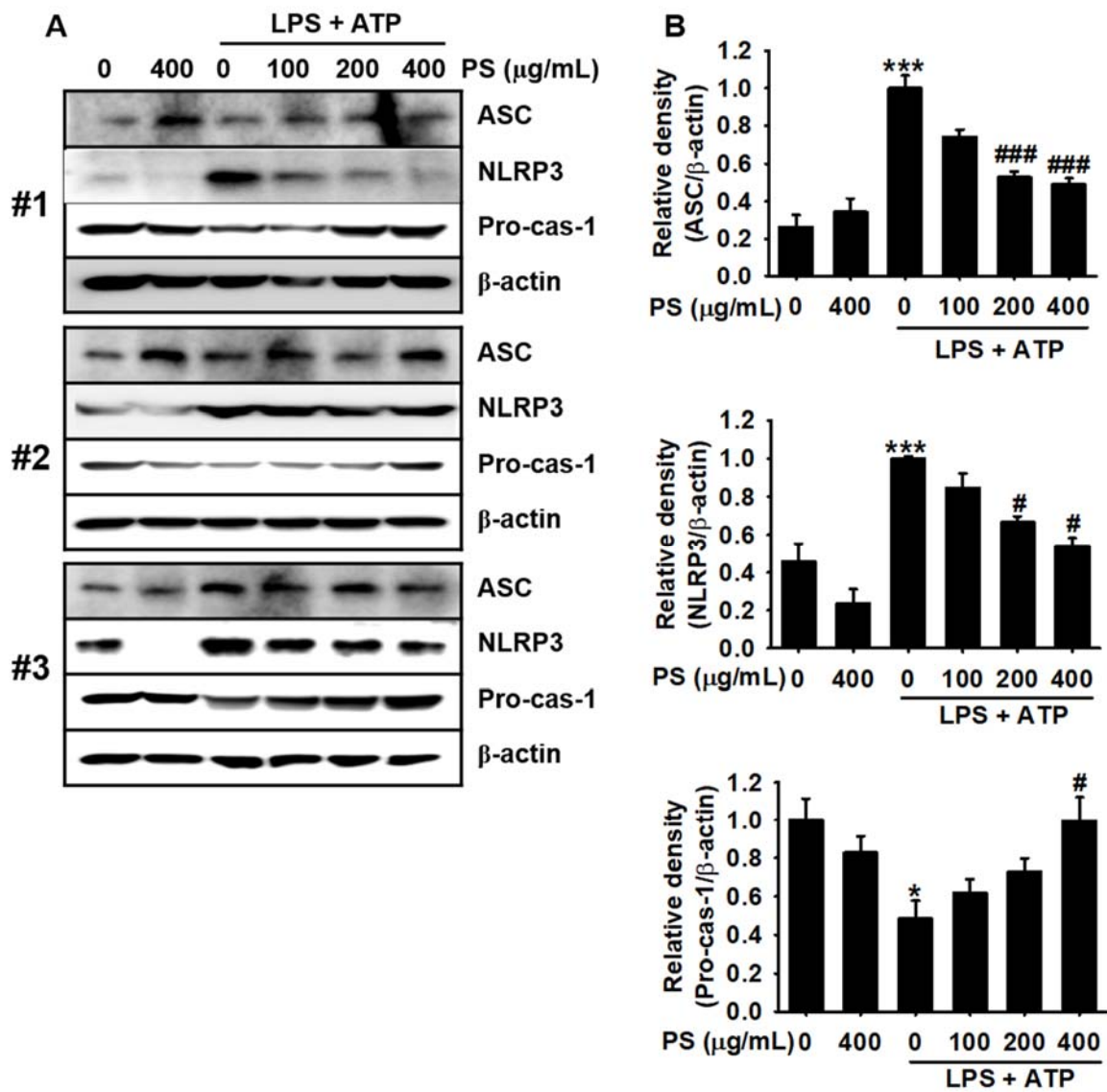
Supplementary Figure S4: Triplicate data (A) and densitometric analysis (B) of Figure 2D.
