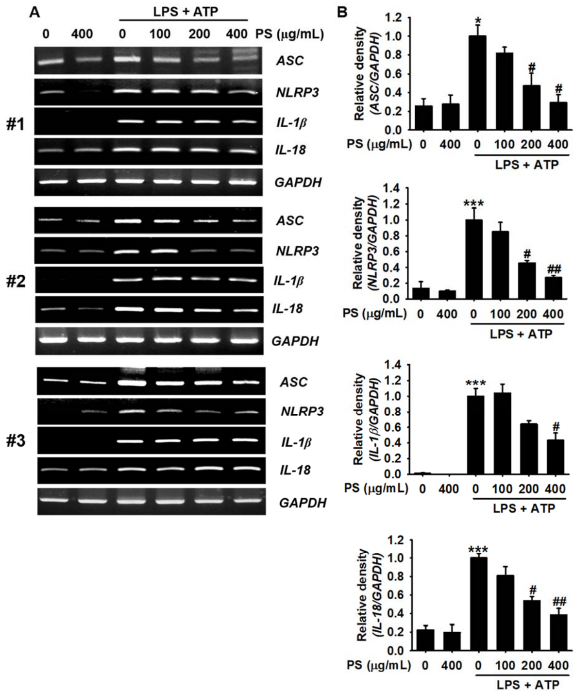
Supplementary Figure S2: Triplicate data (A) and densitometric analysis (B) of Figure 2B.
