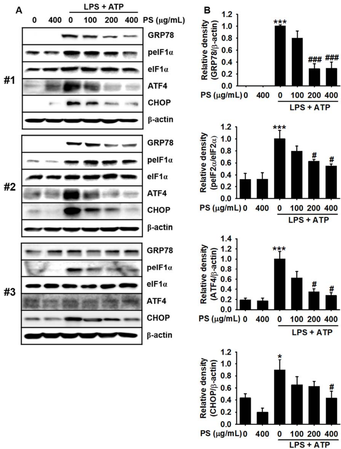
Supplementary Figure S6: Triplicate data (A) and densitometric analysis (B) of Figure 3B.
