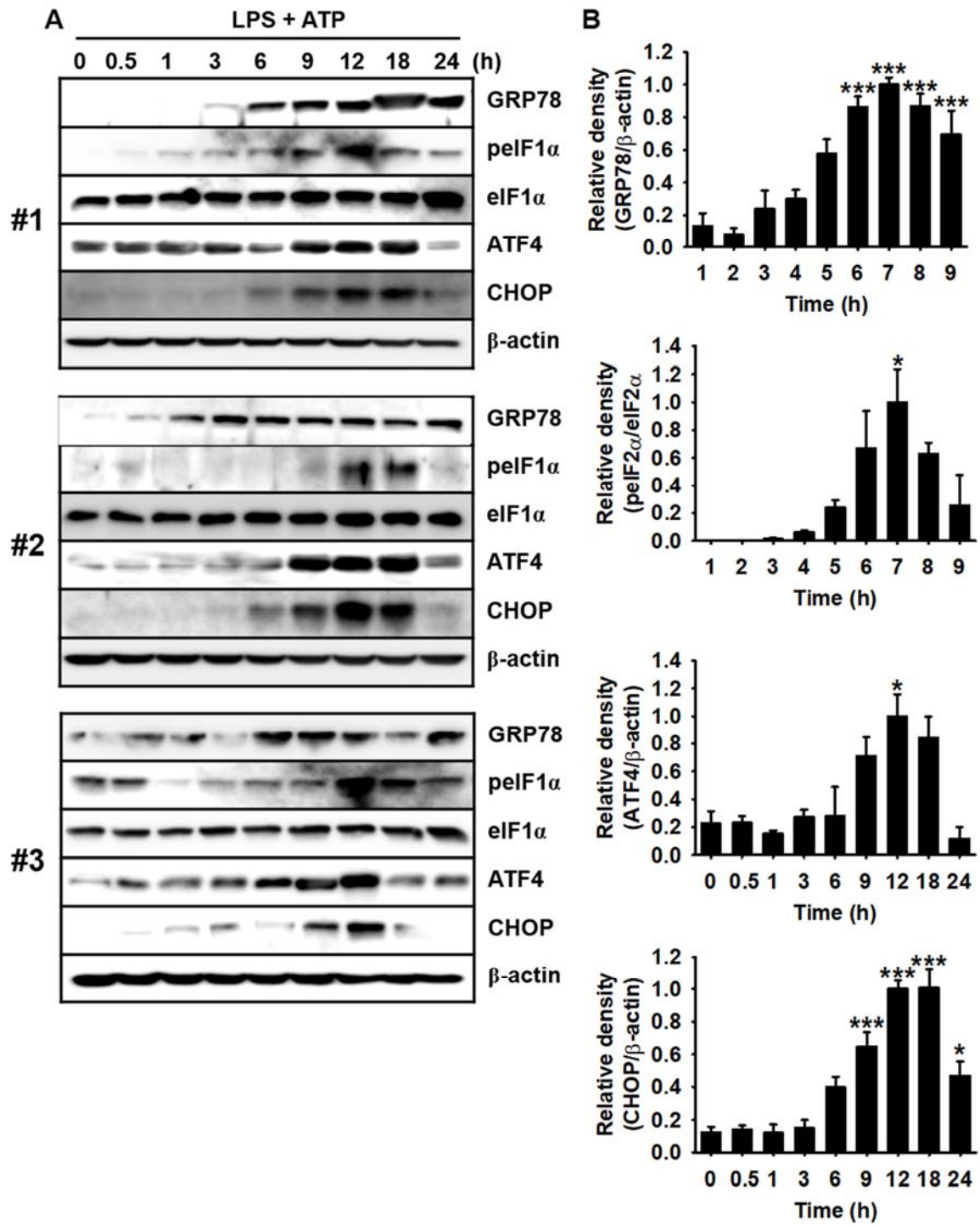
Supplementary Figure S5: Triplicate data (A) and densitometric analysis (B) of Figure 3A.
