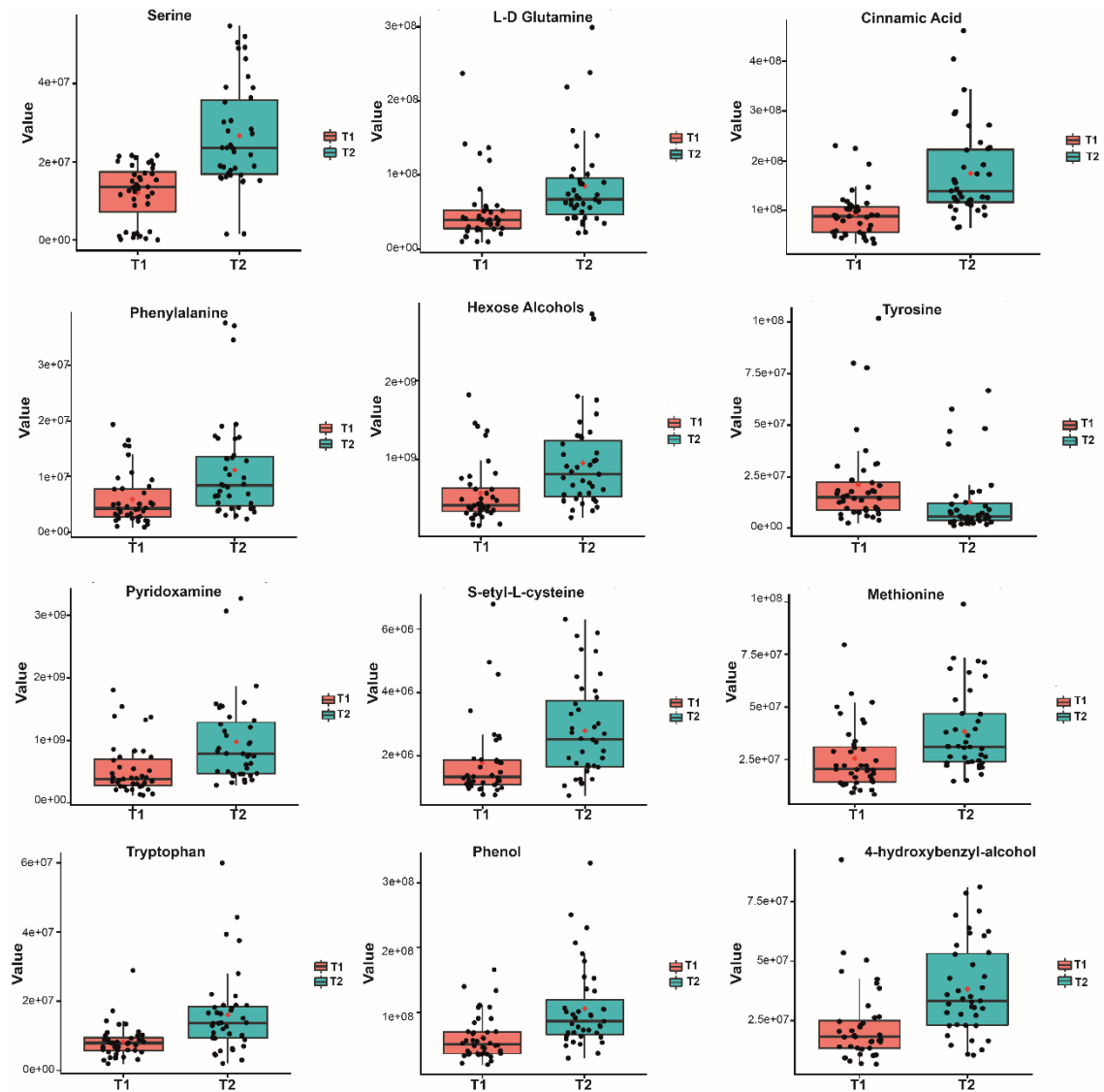
Figure S1: Fecal metabolites whose peak intensity is significantly different between T1 and T2 (p-adjusted < 0.05).
