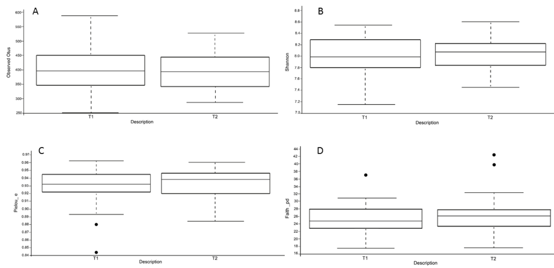
Figure S2: Box plots showing alpha diversity, A) Observed OTUs, B) Shannon Index, C) Pielou's evenness index and D) Faith's Phylogenetic Diversity index in T1 and T2.
