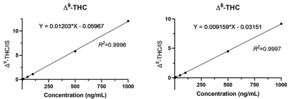
SUPPLEMENTARY FIG. S1. Calibration curves of \Delta^9 -THC and \Delta^8 -THC. \Delta^9 -THC/IS and \Delta^8 -THC/IS ratios plotted against nominal concentration of the calibration standards. Linear equation and R^2 are reported for each plot. IS, internal standard; THC, tetrahydrocannabinol.
