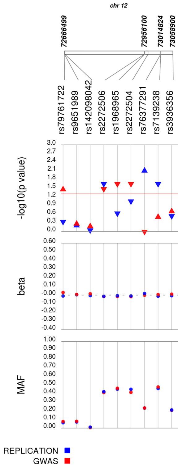
S4 Fig Heterogeneous associations between THRDE variants and M-Index in replication and GWAS dataset. Nine SNPs with minor allele frequency greater than 1% in the replication cohort were included for analysis. Three SNPs were associated with M-Index with P < 0.05 in the replication dataset.
