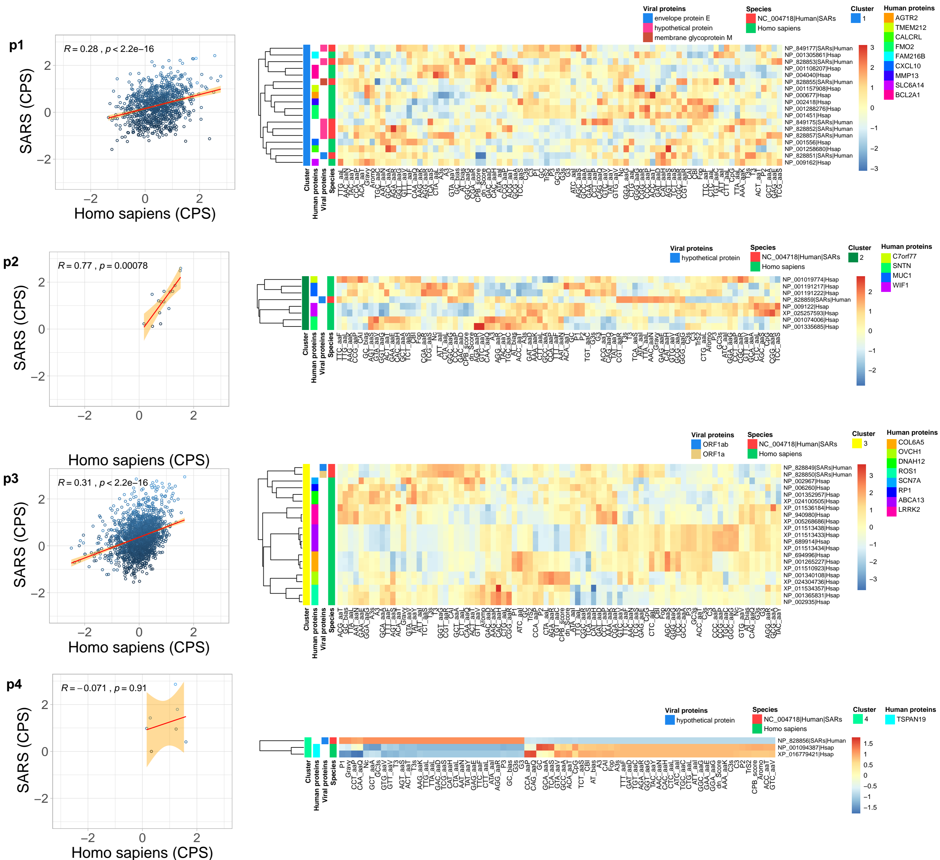
Supplementary file 5: Heatmap of clusters (1 to 4) using hierarchical method of viral genes for SARS (NC_004718) of human host and human genes based on the molecular features. CPB correlation is included in the left for each cluster relating the CPB of human genes (horizontal axis) and CPB of the viral genes (vertical axis).
