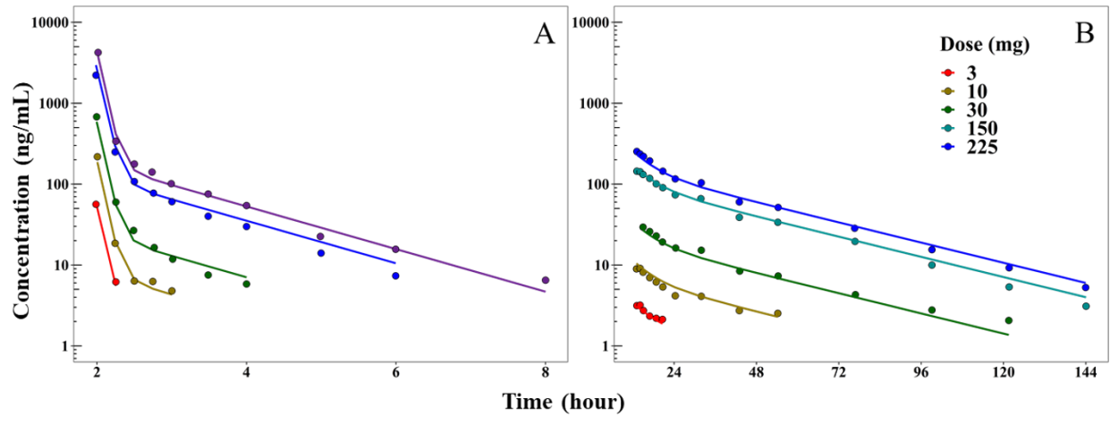
Figure S2. Human Pharmacokinetic Model Fits. Semi-log plot of concentration of mean remdesivir and its nucleoside metabolites versus time in healthy human volunteers following a single 2-hour intravenous infusion of remdesivir. Model fits (lines) of observed data (points) are shown for total plasma concentration of (A) remdesivir and (B) nucleoside after a single dose.
