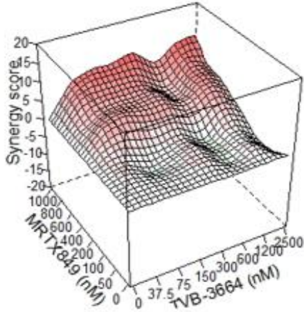
C H460 Average synergy: 0 (Bliss)
