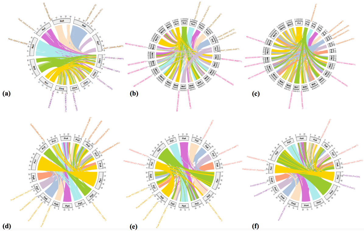
Figure S4. Inter-genomic synteny blocks between species. Comparisons include (a) A. thaliana vs R. occidentalis , (b) R. occidentalis vs M. domestica , (c) M. domestica vs P. avium , (d) P. avium vs P. persica , (e) P. persica vs P. armeniaca , and (f) P. armeniaca vs P. mume .
