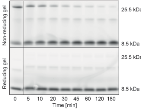
N \alpha -acetyl-L-Lysine
