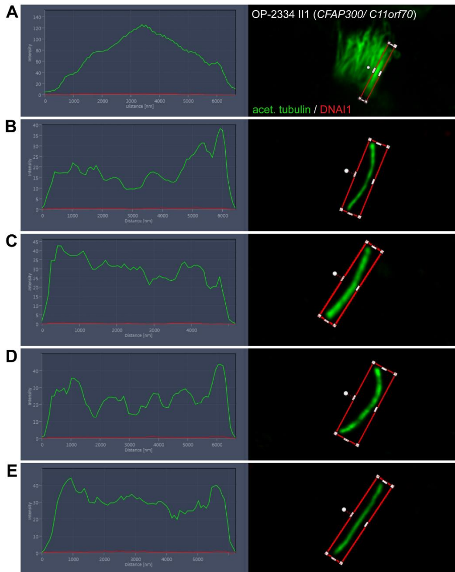
S16 Fig. Measurement of the DNAI1 fluorescence intensity along the ciliary axonemes of CFAP300/C11orf70 -mutant respiratory cells. Intensity profile of DNAI1 signal (red) shows absence of DNAI1 in ciliary axonemes of CFAP300/C11orf70 -mutant cilia (OP-2334) when compared to control cells (S11 Fig). The red boxes indicate the path of the intensity profile. Five representative examples are shown.
