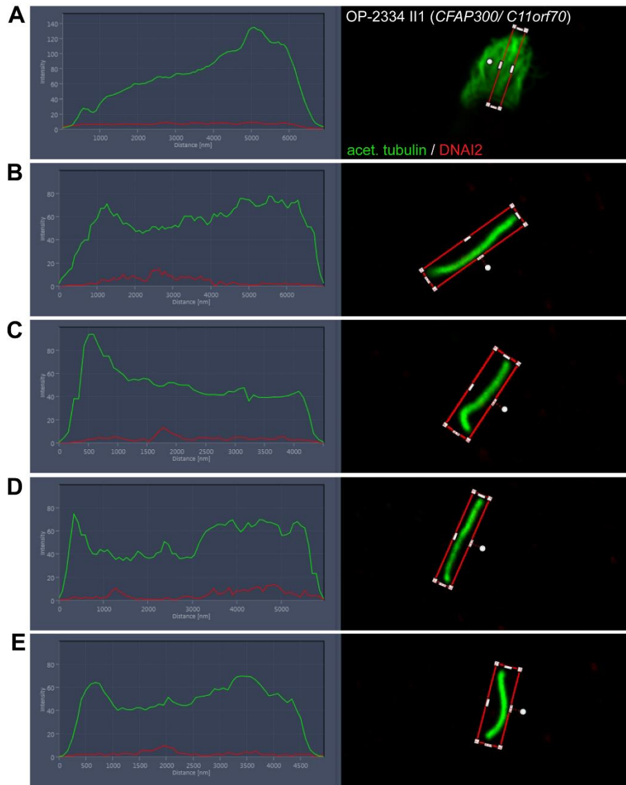
S24 Fig. Measurement of the DNAI2 fluorescence intensity along the ciliary axonemes of CFAP300/C11orf70 -mutant respiratory cells. Intensity profile of DNAI2 signal (red) shows absence or severe reduction of DNAI2 in ciliary axonemes of CFAP300/C11orf70 -mutant cilia (OP-2334), when compared to control cells (S19 Fig). The red boxes indicate the path of the intensity profile. Five representative examples are shown.
