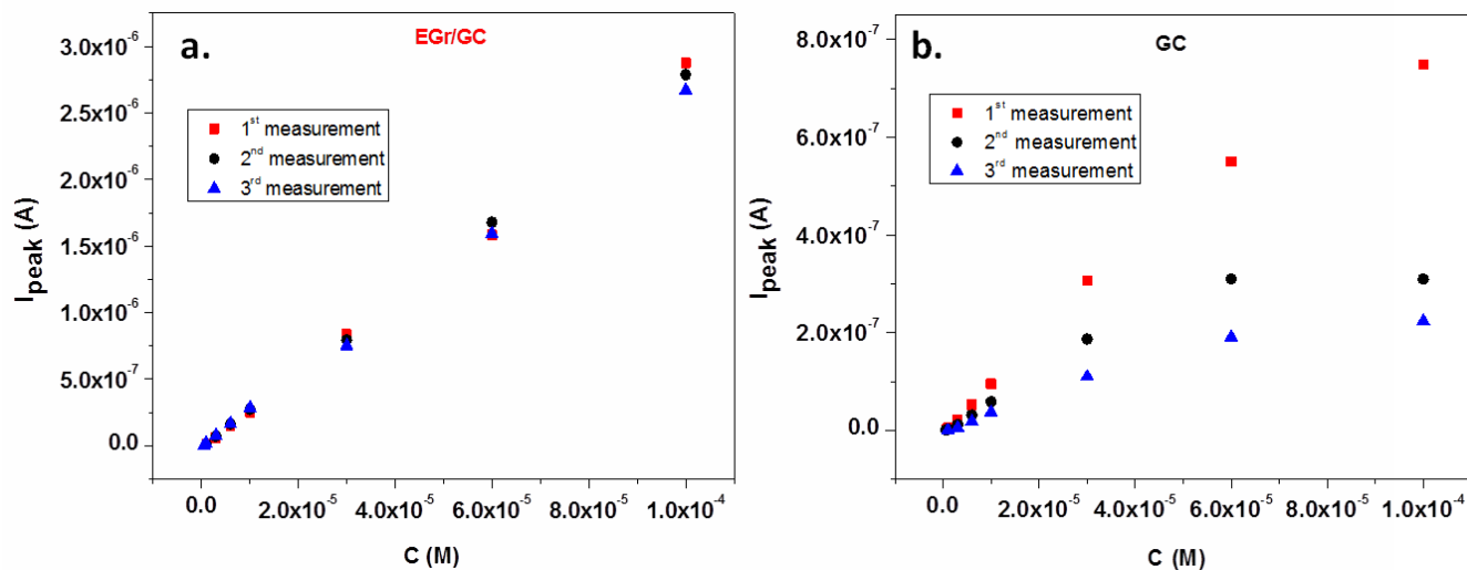
Figure S1. Calibration plots obtained from 3 successive measurements recorded with EGr/GC (a) and GC (b) electrodes.
