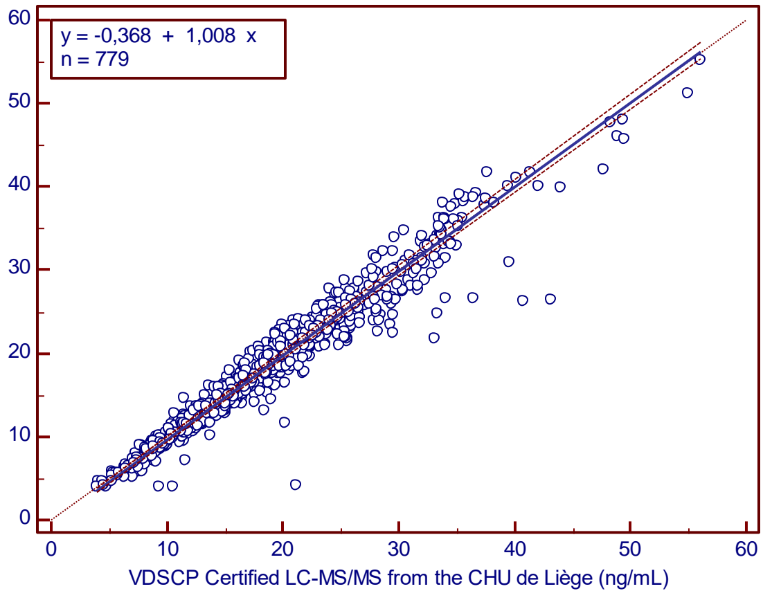
Supplementary Figure S1. Passing-Bablok regression of 25(OH)D values (ng/mL) obtained with the Fujirebio Lumipulse and the VDSCP-certified LC-MS/MS of the CHU de Liège. 25(OH)D: twenty-five-hydroxy vitamin D; VDSCP: Vitamin D Standardization-Certification Program; LC-MS/MS: liquid chromatography tandem mass spectrometry.
