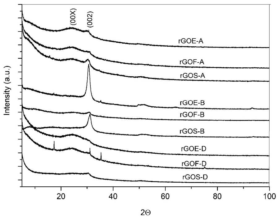
Figure S5. XRD spectra of reduced graphene oxides.
