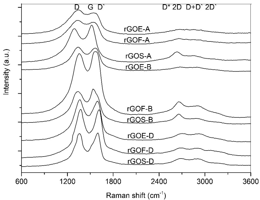
Figure S3. Raman spectra of reduced graphene oxides.
