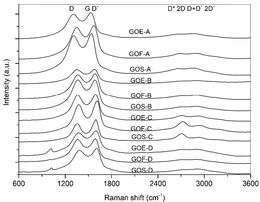
Figure S2. Raman spectra of graphite oxides.
