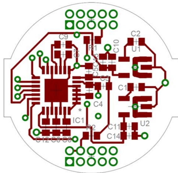
Figure 8. ECG sensor board schematics and layout – ECG signal conditioning is based on MAX30003 analog frontend.
