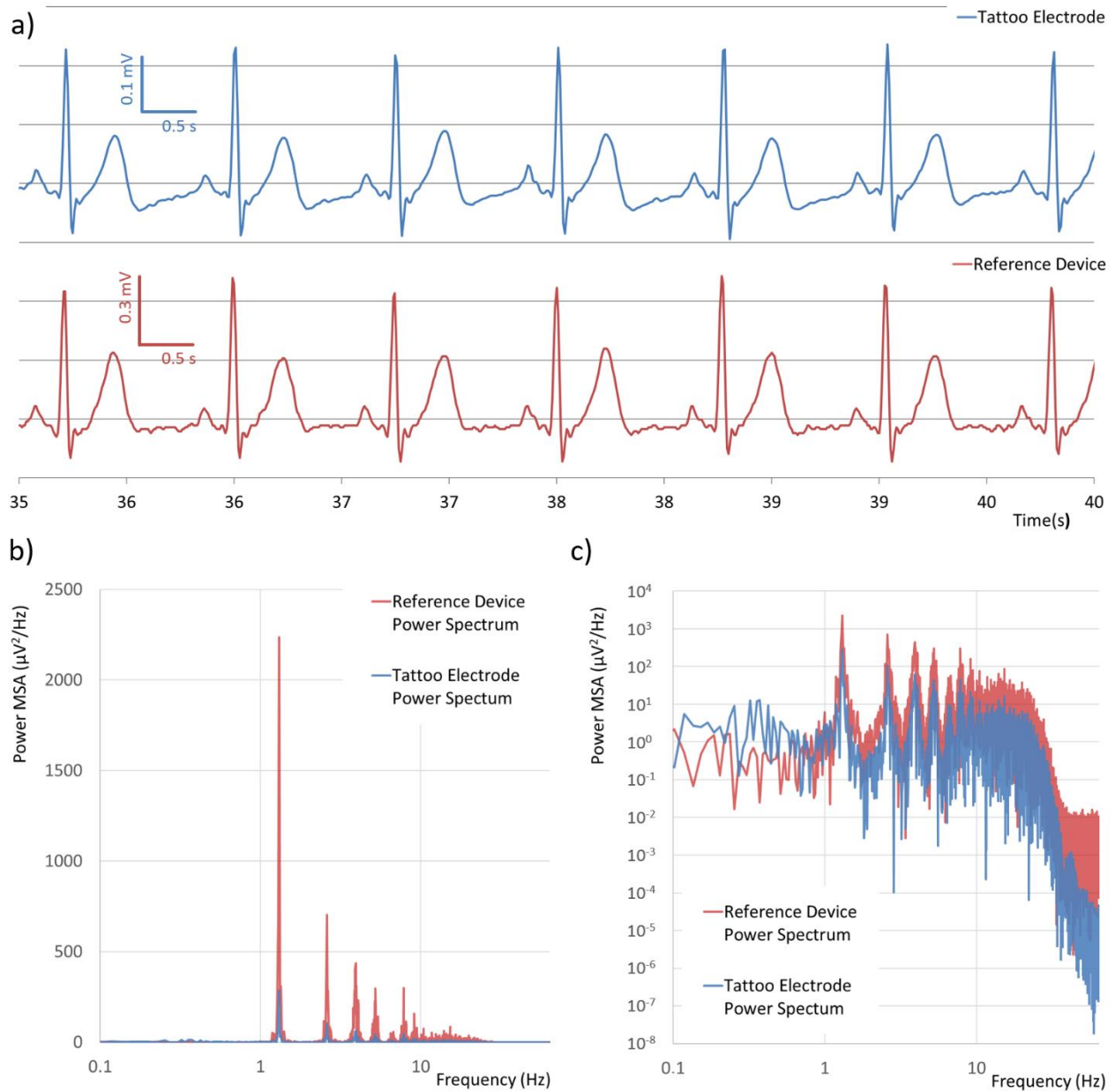
Figure 9. a) Detail of ECG acquisition from tattoo electrodes by BLE device and reference device with standard electrodes; (b) Power spectrum at mean squared amplitude(MSA) of the ECG signal calculated on 60 seconds sample, both for tattoo electrode + BLE device and reference device; (c) same spectrum with different logarithmic scaling, for clarity of comparison.
