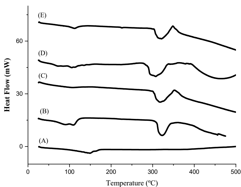
Figure S1. DSC thermogram (A) Perillyl alcohol, (B) \beta -cyclodextrin, (C) Co-evaporation, (D) Malaxation and (E) Physical mixture.
