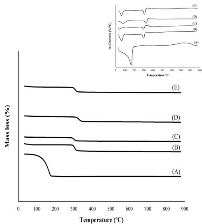
Figure S2. TG/DTGG curves of (A) Perillyl alcohol, (B) \beta -cyclodextrin, (C) Co-evaporation, (D) Malaxation and (E) Physical mixture.
