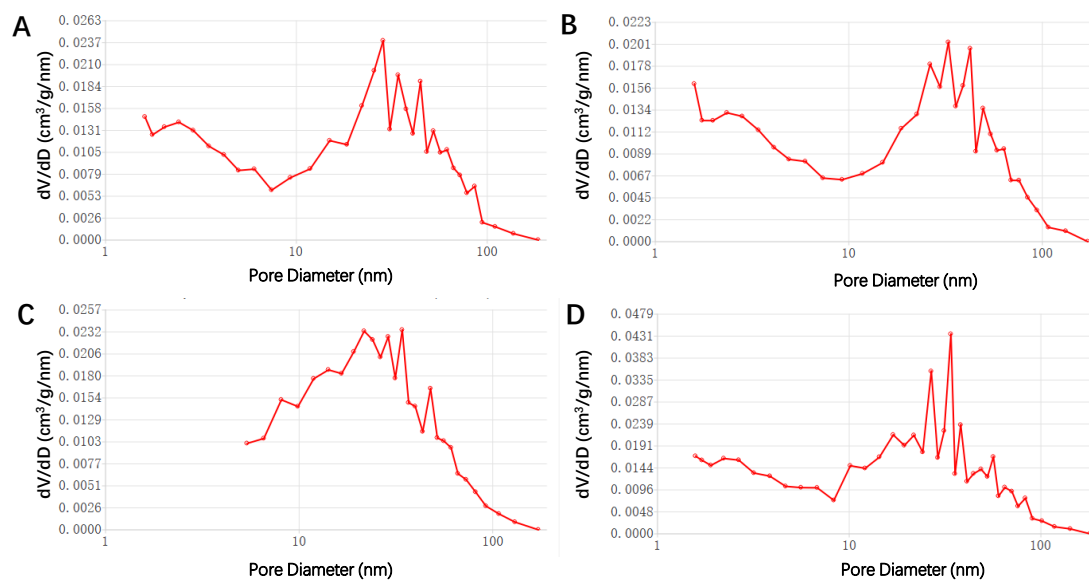
Figure S1. Pore distribution of (A) OCBs-1, (B) OCBs-2, (C)OCBs-3 and (D)OCBs-4.
