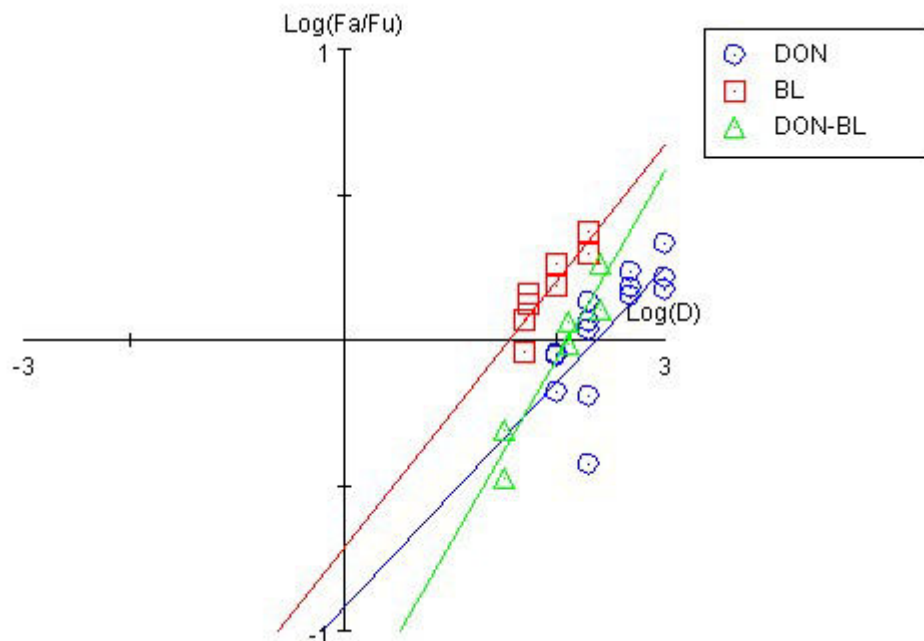
Median-Effect Plot
