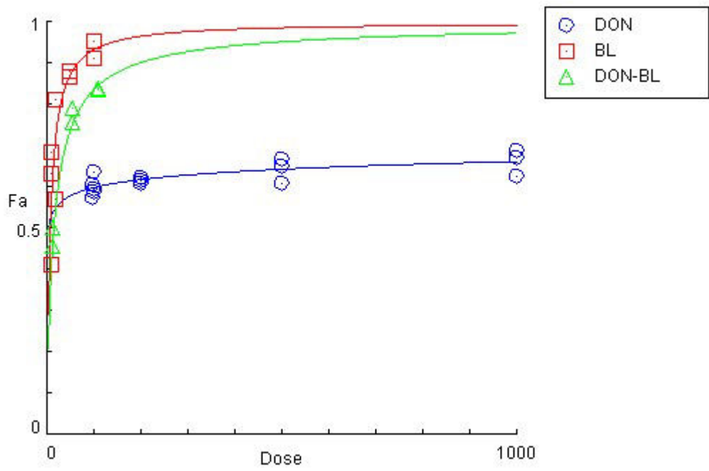
Dose-Effect Curve
