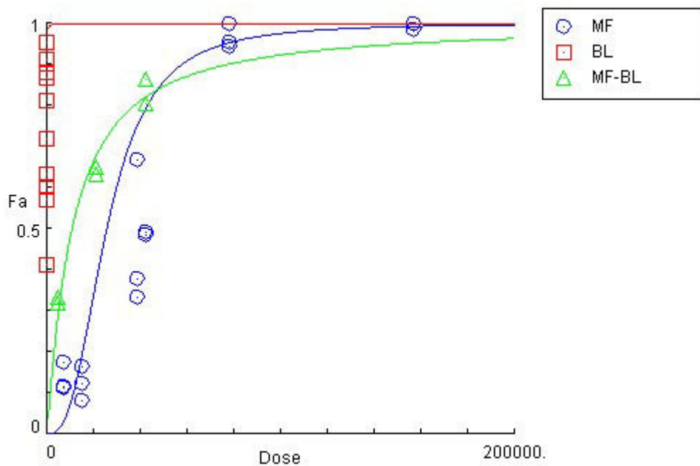
Dose-Effect Curve
