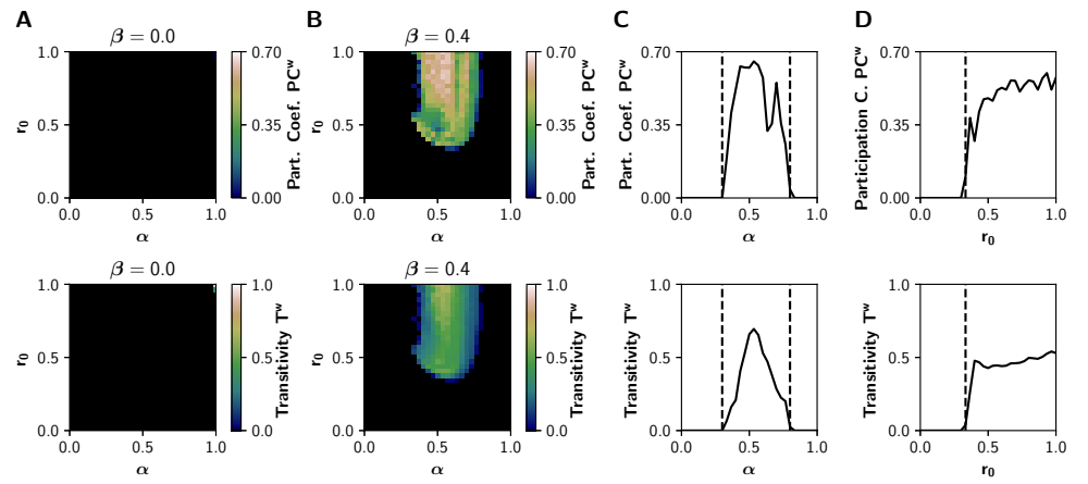
S3 Fig. Alternative measures of network segregation and integration in the (\alpha, r_0) parameter space for \beta = 0.4 .
