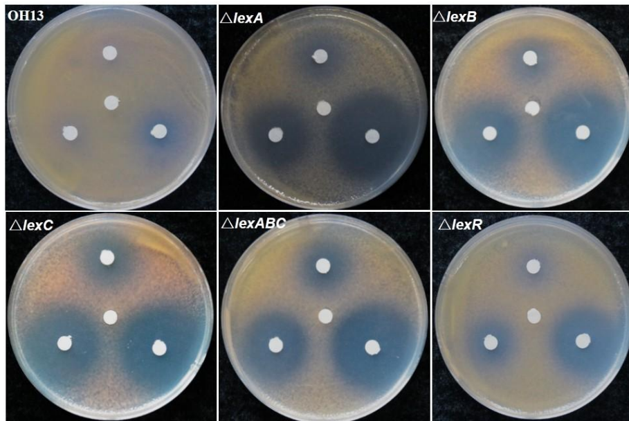
FIGURE S3 Inhibition assay of myxin against L. antibioticus OH13, lexA , lexB , lexC , lexABC , lexR mutants. On a plate, center, negative control; top, 0.125 \mu\text{g} myxin; left, 0.25 \mu\text{g} myxin; right, 0.5 \mu\text{g} myxin.
