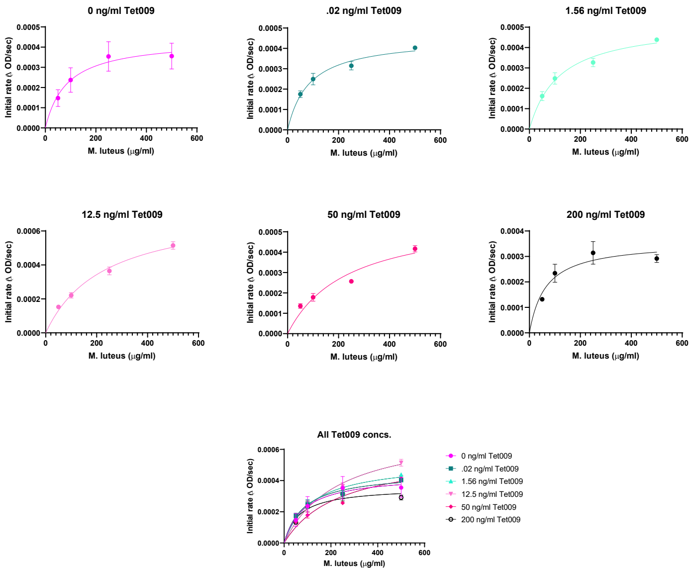
Fig. S2 - Pseudo-Michaelis-Menten kinetic analysis of hLYS lytic rates towards Gram-positive M. luteus bacteria in the presence of the specified concentration of Tet009 AMP. All reactions were evaluated in triplicate and shown are the means and standard deviation of the initial rate at each bacterial substrate concentration. The best fit hyperbola for each data set is shown, and V_{max} values from the regressions are provided in Fig. 3.
