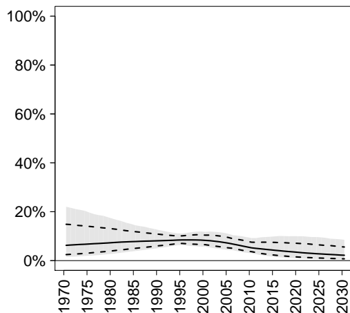
CP (traditional)
