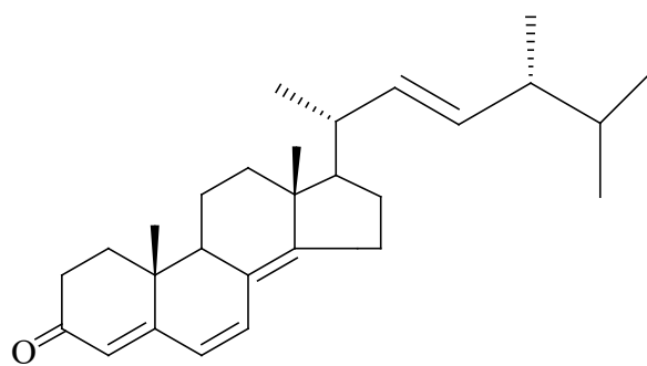
Figure S1 Chemical structure of ergone.
