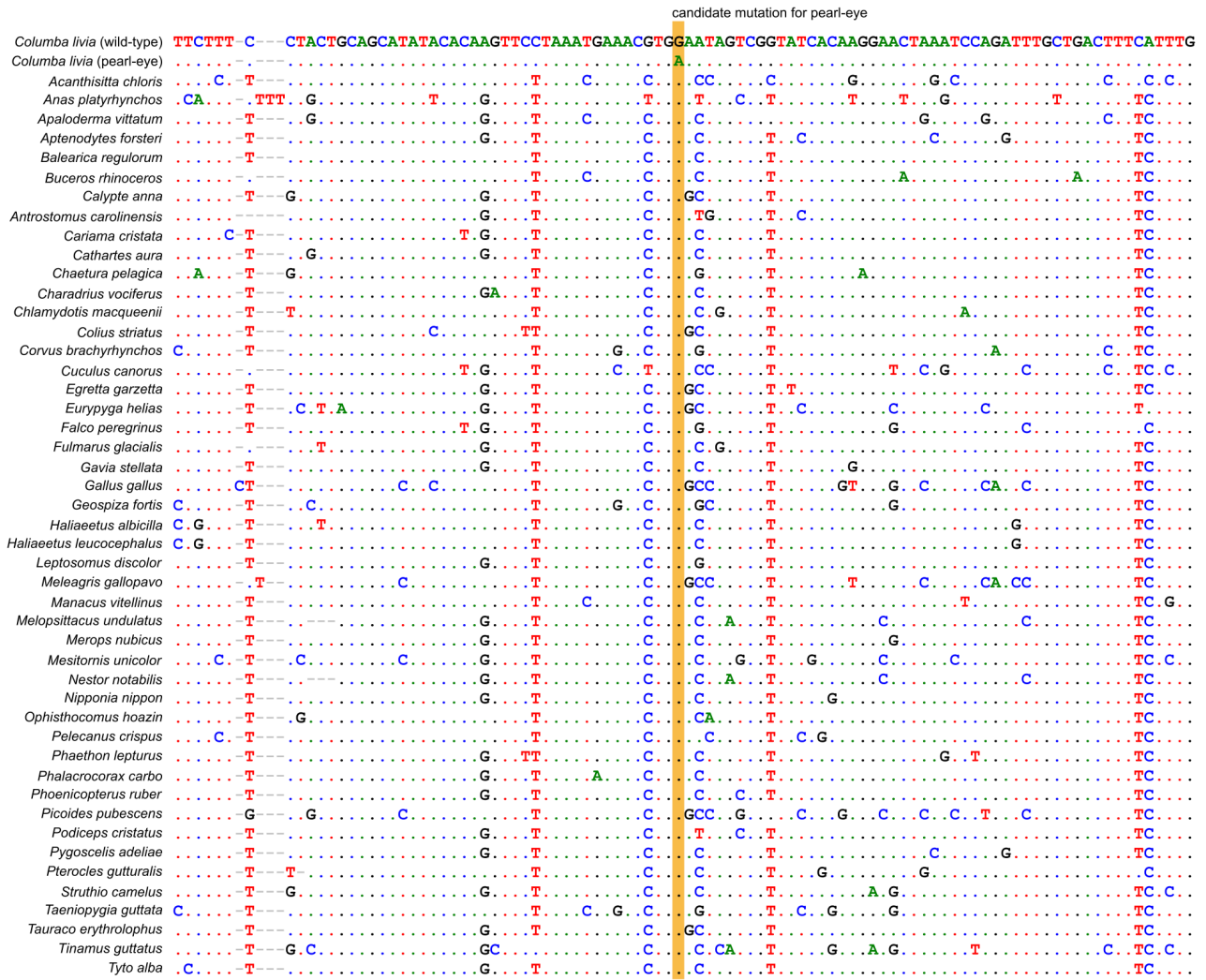
S1 Fig. Alignment of multiple bird genomes in the candidate nonsense mutation region. The candidate mutation is highlighted in orange.
