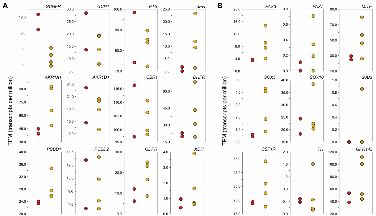
S3 Fig. Gene expression profiles between pearl-eye (red) and wild-type (yellow) pigeons for candidate genes for skin color development in ectothermic vertebrates. (A) Relative expression levels (TPM, transcripts per million) of genes in the pterin synthesis pathway. (B) Similar to panel (A) for a group of genes previously implicated in xanthophore differentiation in ectothermic vertebrates.
