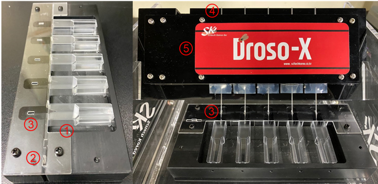
Supplementary Fig. S1. Details of Droso-X machine. ① A cuvette which houses a single fly. ② A blocker which can be controlled to start feeding. ③ A hole through which the glass tube passes. ④ A glass tube which contains food. ⑤ Droso-X machine with sensors.
