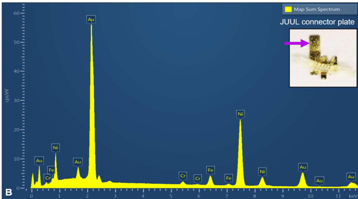
S2 Fig. EDS spectra of JUUL atomizer components. (A) wick, which comprises silicon and oxygen, and (B) the connector plate, mainly nickel coated with gold. The Blue arrow indicates the wick, and the purple arrow indicates the connector plate.
