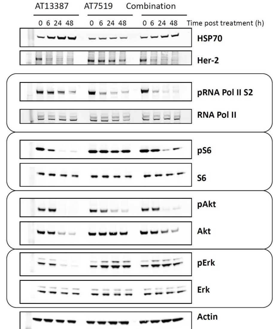
Supplemental Figure 1. In vitro suppression of HSP90 inhibitor-dependent HSP70 induction with increasing concentrations of AT7519 and modulation of select client proteins by western blot.
