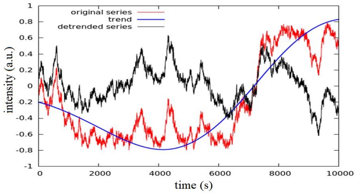
S2 Fig. Trend removal using Empirical Mode Decomposition.
