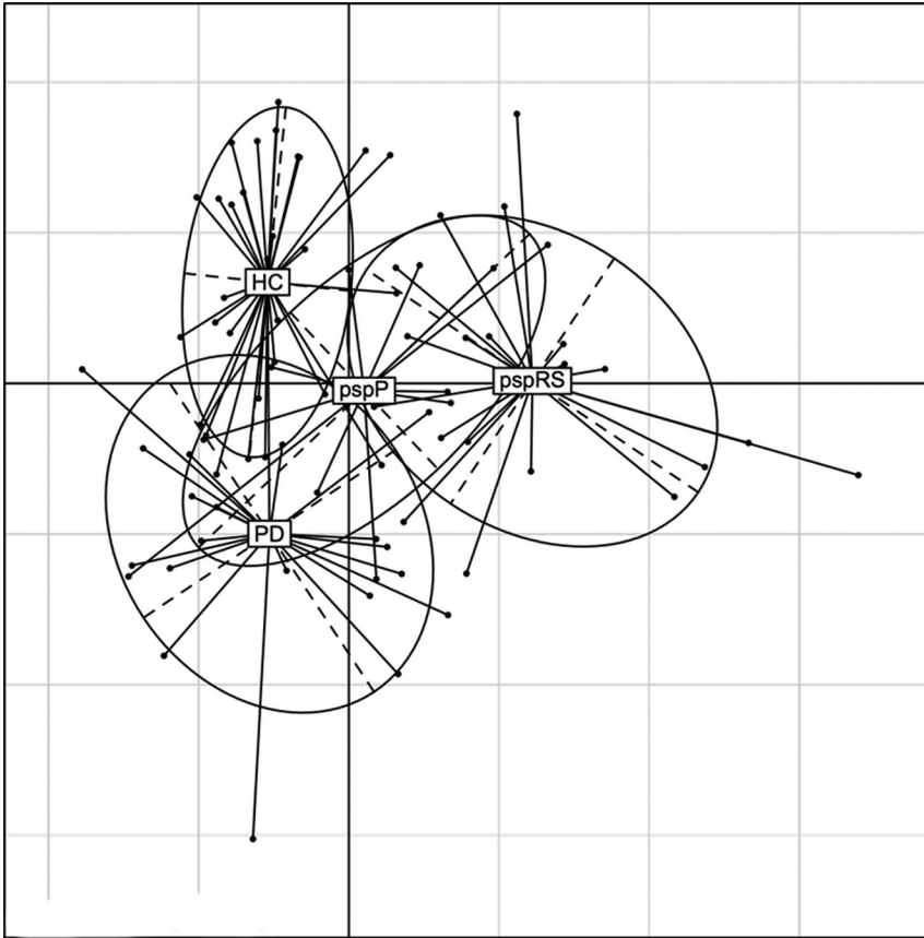
ON-LINE FIG 1. Data projected onto the plane defined by the linear discriminant components. Each ellipse represents a study group, where the center indicates between-variances, while the area is proportional to the within-variances.
