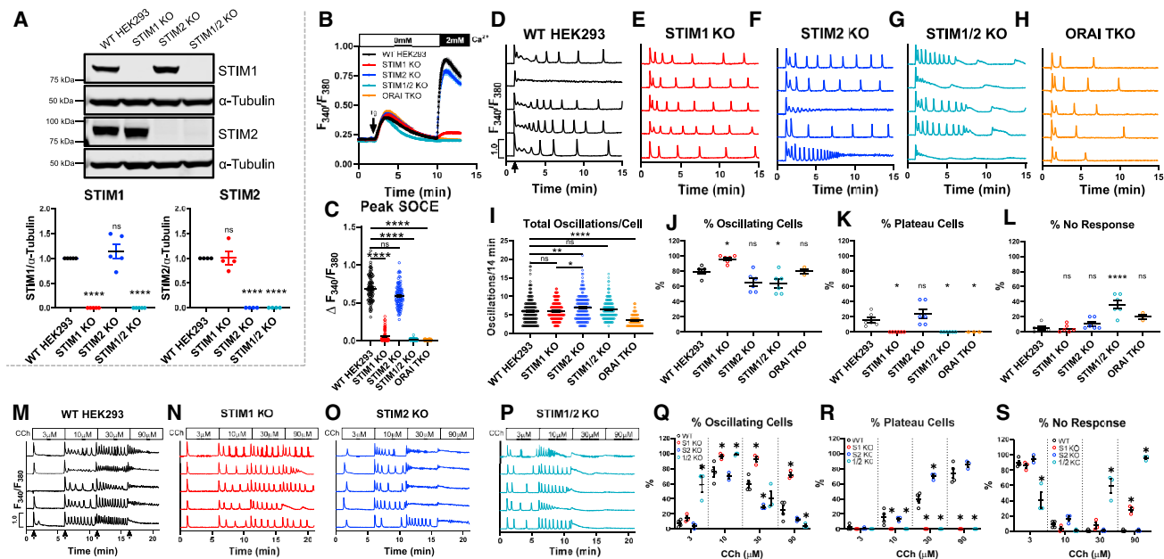
Figure 1. Native STIM1/STIM2 mediate unique Ca^{2+} oscillation profiles and agonist sensitivities
