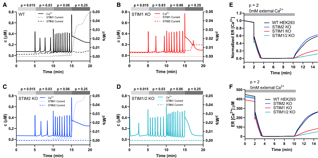
Figure 6. Mathematical modeling supports coordinated STIM1/STIM2 functions over the diverse range of \text{Ca}^{2+} signaling events
