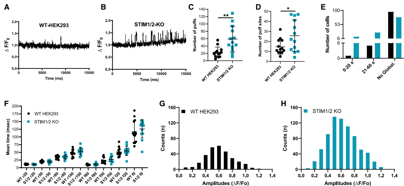
Figure 5. STIM1/STIM2 regulate IP 3 R-mediated Ca 2+ puffs in response to IP 3 uncaging
