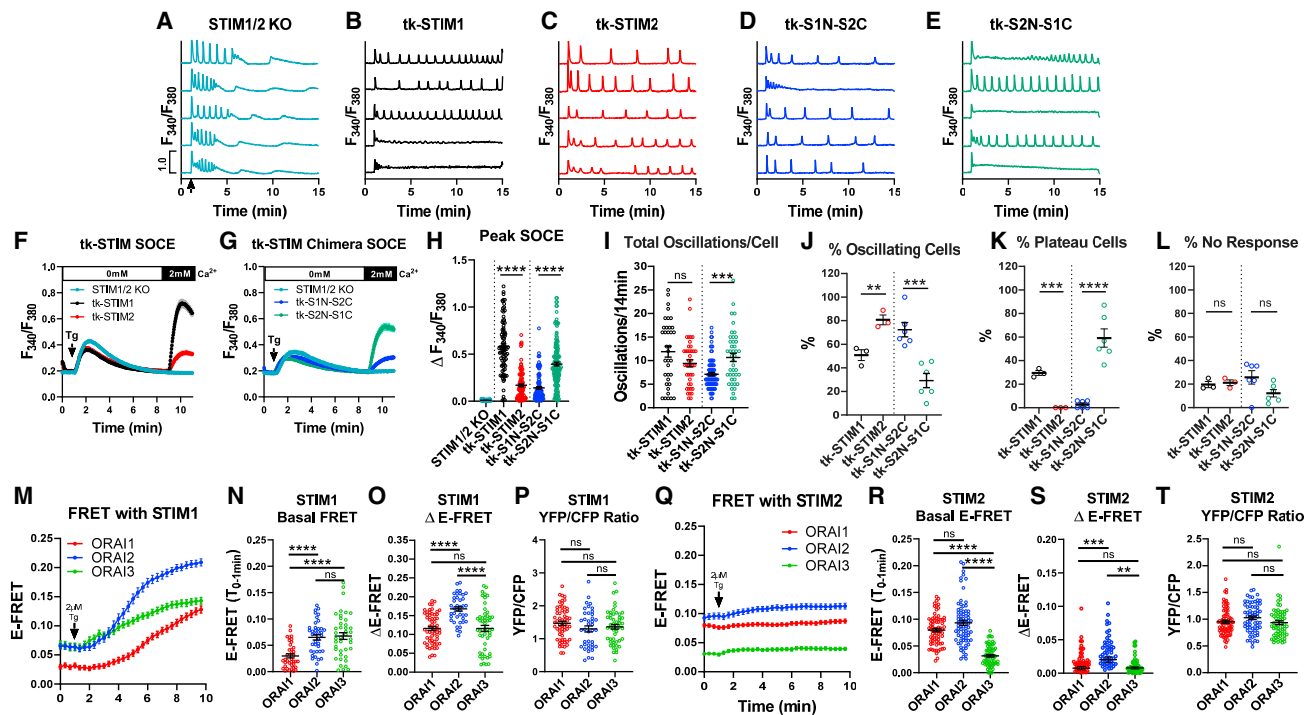
Figure 2. STIM1/STIM2 have distinct interactions with Orai1/2/3
