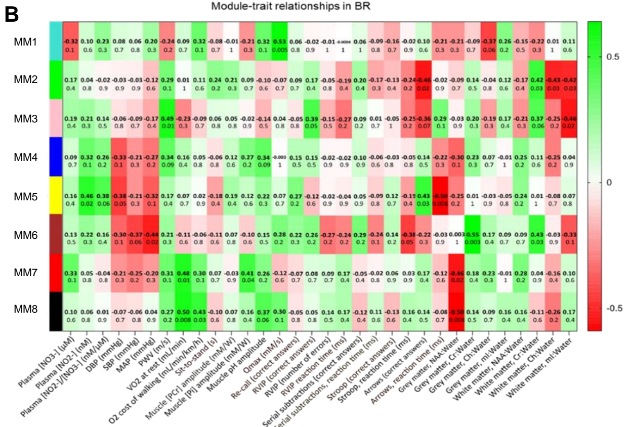
Fig. S2. Eigengene correlation networks between oral microbiome modules (MM1-MM8; vertical axis) versus 32 physiological and cognitive traits (horizontal axis) within placebo (PL; A) and nitrate (BR; B) conditions. The colour scale on the right-hand side of each panel indicates the strength of positive (green) and inverse (red) correlations
