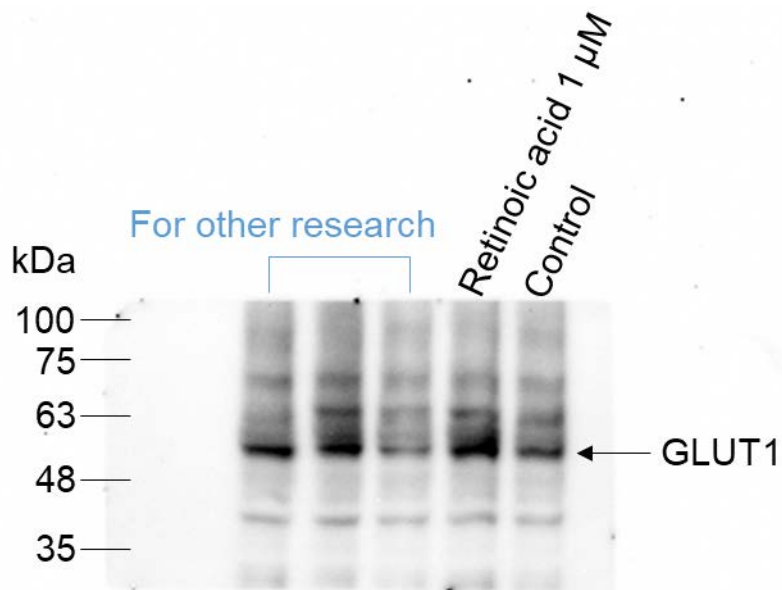
S1 Fig. Full-length gels and blots. The GLUT1 protein has a size of 55 kDa but varies slightly in shape depending on cell, antibody or experimental conditions.
