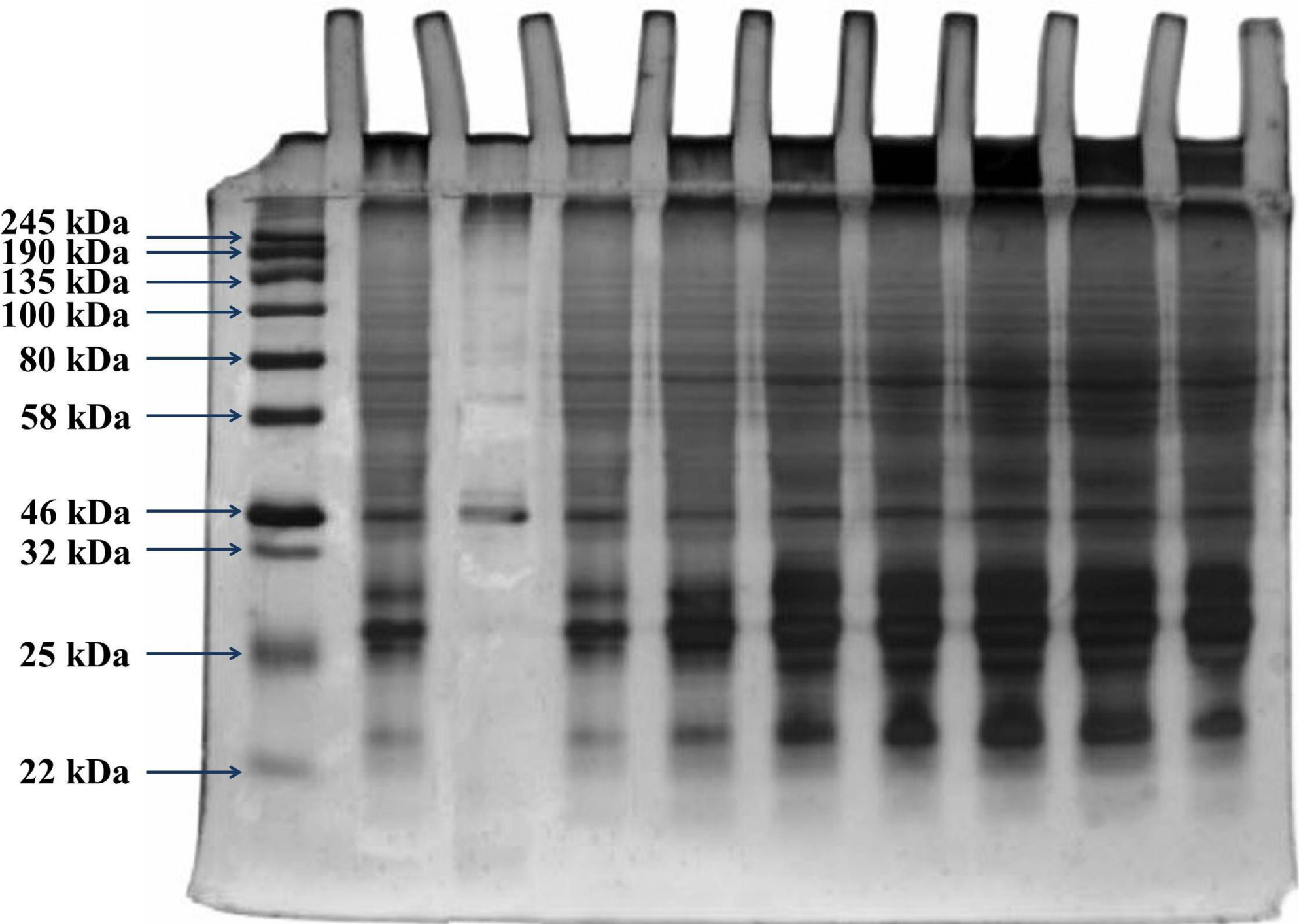
Figure 6(b) SDS-PAGE analysis of Mang Mao wings extract protein; Lane 1. Molecular size marker; lane 2. Crude protein; lane 3. Purified protein (46 kDa) responsible for active biosynthesized MMAgNPs
