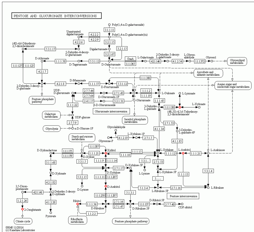
Figure S7 Effects of xylitol on pentose and glucuronate interconversion metabolites in vitro (Red-up regulate, Blue-down regulate).
