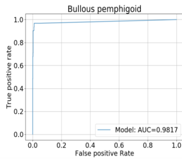
Supplementary Figure 1: Representative ROC plots for all 20 skin conditions showing the AUC values from fold 0
