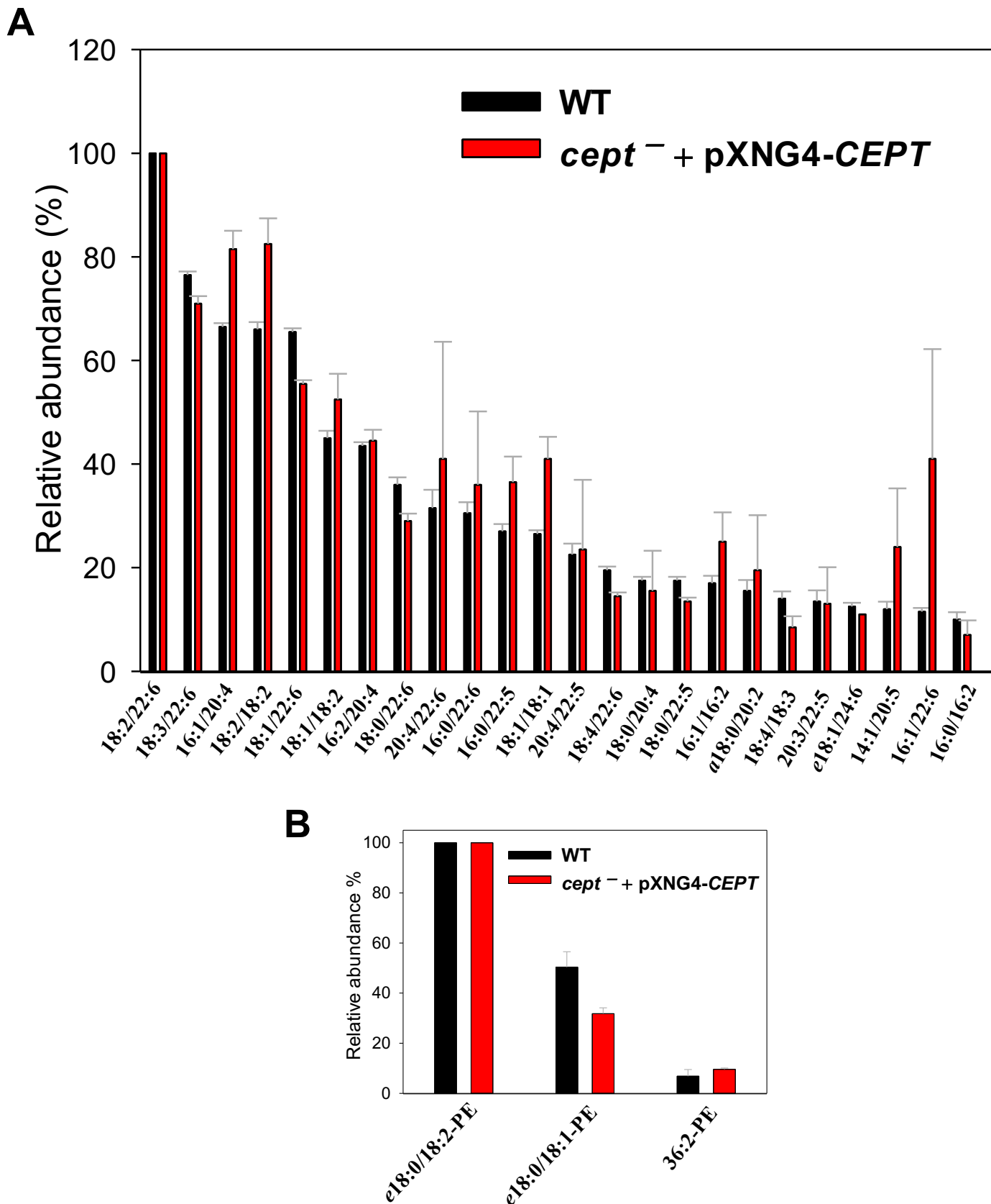
Figure S4. Cept - +pXNG4-CEPT promastigotes show similar phospholipid composition as WT promastigotes. Lipids from log phase promastigotes were analyzed by ESI-MS in the positive ion mode (A: for PC) and negative ion mode (B: for PE). Predicted fatty acyl constituents were indicated. Only major PC and PE species (>5% by relative abundance) are shown.
