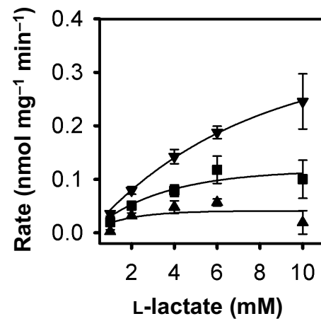
Figure S4. Michaelis-Menten kinetics for MCT1 fused with BSG variants. Shown are curves for BSGΔIg (■), BSG Ig-I/C2 (▼), BSG var2 (▲). The data were normalized to 1 mg of cells and the background of non-expressing cells was subtracted. Error bars indicate \pm S.E.M. from three biological replicates.
