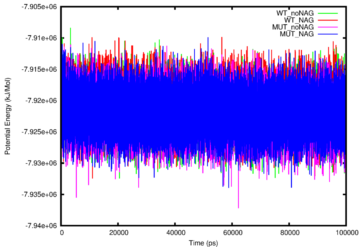
S2 Fig. Potential energy of the four systems of NRXN2 (WT_noNAG, MUT_noNAG, WT_NAG and MUT_NAG) over 100 ns.
