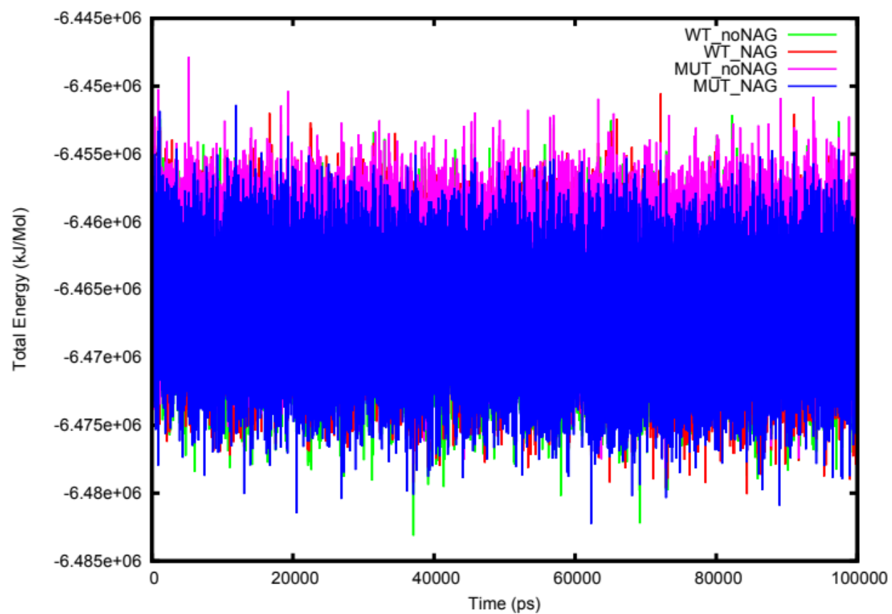
S5 Fig. Total energy of the four systems of the repeat 1 of NRXN2 (WT_noNAG, MUT_noNAG, WT_NAG and MUT_NAG) over 100 ns.
