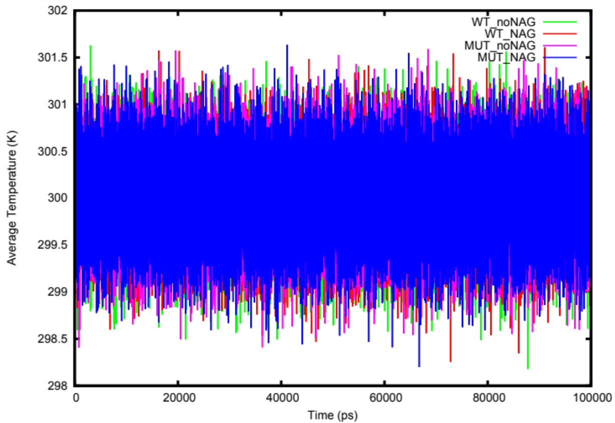
S7 Fig. The average temperature of the four systems of repeat 1 NRXN2 (WT_noNAG, MUT_noNAG, WT_NAG and MUT_NAG) over 100 ns.
