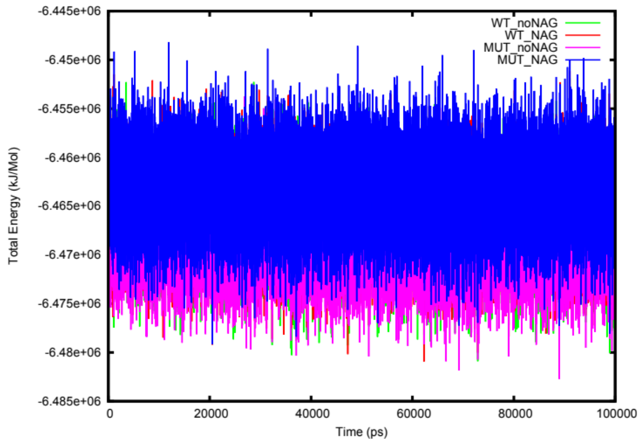
S9 Fig. Total energy of the four systems of the repeat 2 of NRNX2 (WT_noNAG, MUT_noNAG, WT_NAG and MUT_NAG) over 100 ns.
