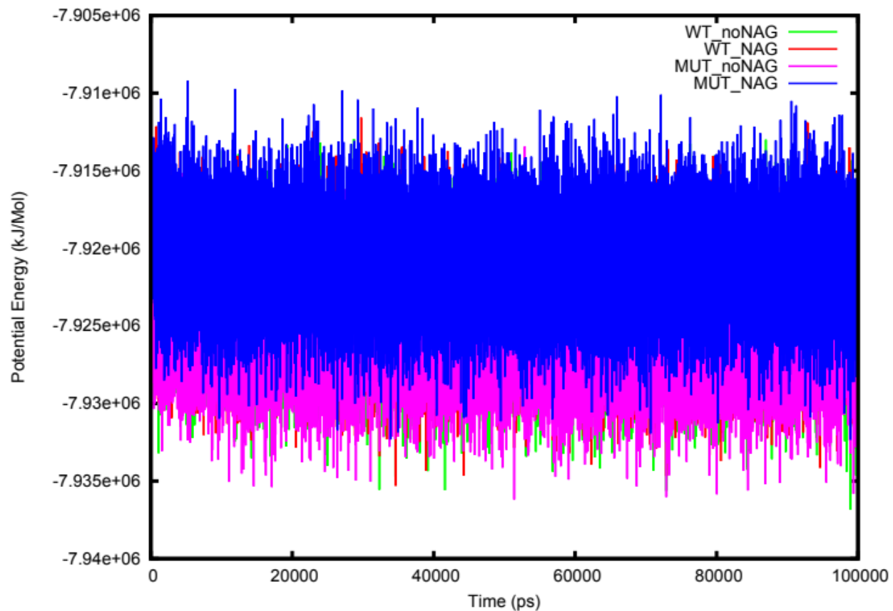
S10 Fig. Potential energy of the four systems of repeat 2 of NRNX2 (WT_noNAG, MUT_noNAG, WT_NAG and MUT_NAG) over 100 ns.
