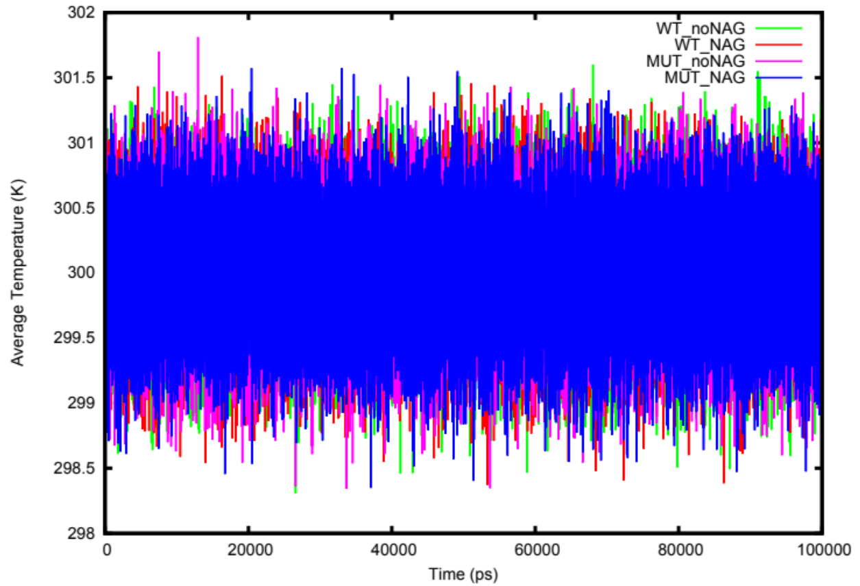
S11 Fig. The average temperature of the four systems of repeat 2 NRNX2 (WT_noNAG, MUT_noNAG, WT_NAG and MUT_NAG) over 100 ns.
