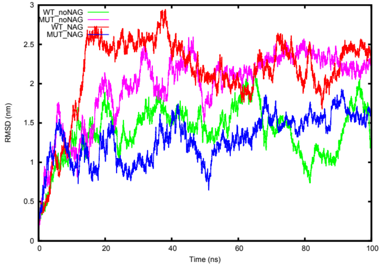
S12 Fig. RMSD deviation of the backbone atoms for the four systems of repeat 2 NRXN2, ( 1.40\text{nm} \pm 0.33 , 1.98\text{nm} \pm 0.45 , 2.15\text{nm} \pm 0.51 and 1.29\text{nm} \pm 0.29 ). Line colors: WT_noNAG = green, MUT_noNAG = light magenta, WT_NAG = red and MUT_NAG = blue.
