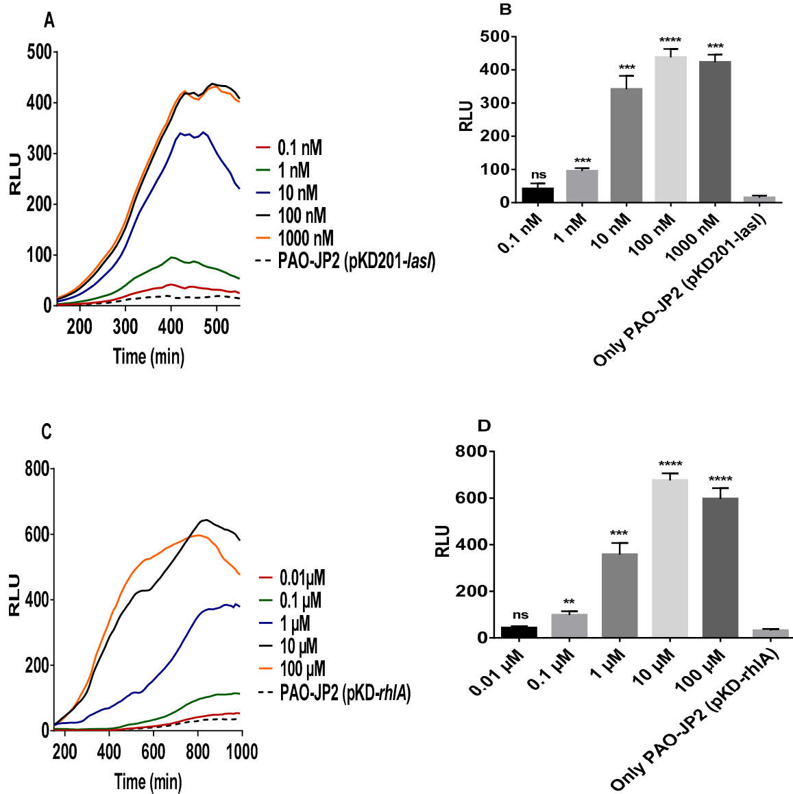
Figure S1. Induction of bioluminescence. (A) Bioluminescence emission of PAO-JP2 (pKD201- lasI ) in the presence of different concentrations of 3-oxo-C12-HSL. (B) Bioluminescence induction relative to the control, corresponding to the data in panel A. (C) PAO-JP2 (pKD- rhlA ) luminescence in the presence of different concentrations of C4-HSL. (D) Bioluminescence induction relative to the control, corresponding to the data in panel C. All concentrations presented are the final concentrations. Luminescence was expressed as relative light units or RLU. ** p < 0.01 , *** p < 0.001 , **** p < 0.0001 , and ns not significant. Values represent mean \pm SD, n = 3 (three experimental readings).
