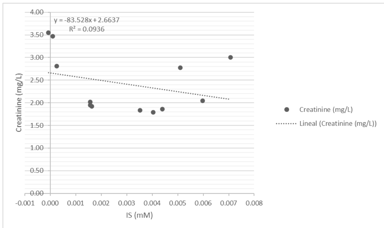
Figure S1. Correlation between creatinine and indoxyl sulfate (IS) levels of the control group.
