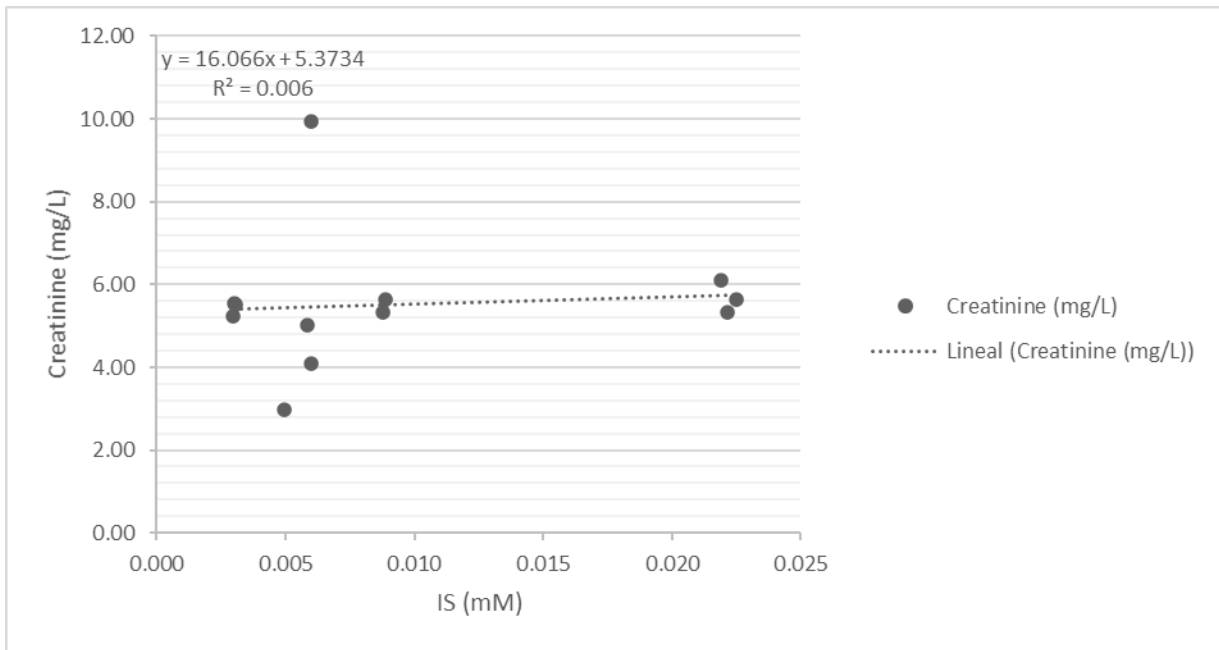
Figure S2. Correlation between creatinine and indoxyl sulfate (IS) levels of the Nef group.
