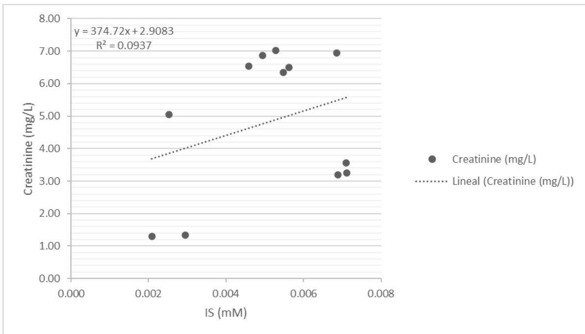
Figure S3. Correlation between creatinine and indoxyl sulfate (IS) levels of the Lac group.
