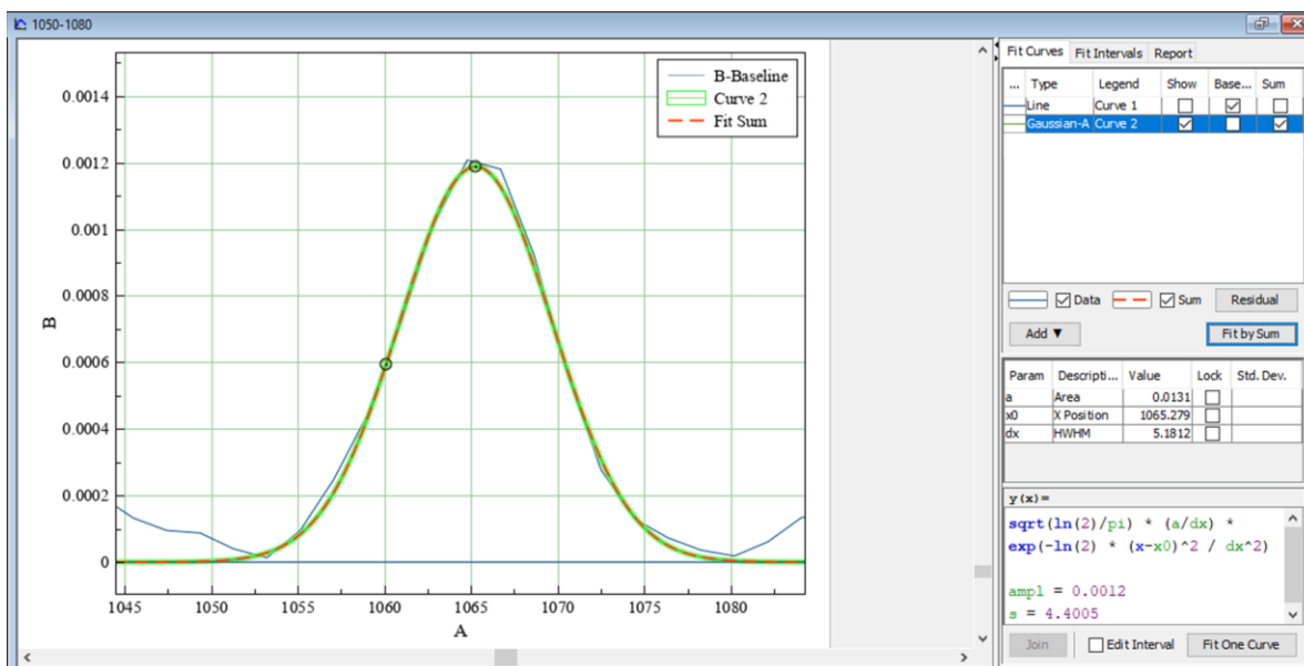
Figure S1. Example of area measurement by MagicPlot software, in wavenumber range 1045–1080 cm -1 , of a Raman spectrum from an arbitrary cartilage sample.
