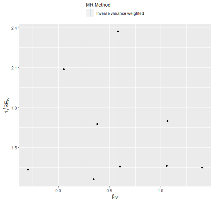
Supplementary Figure 1 | The funnel plot. The symmetry of the funnel plot explains the absence of horizontal pleiotropy.
